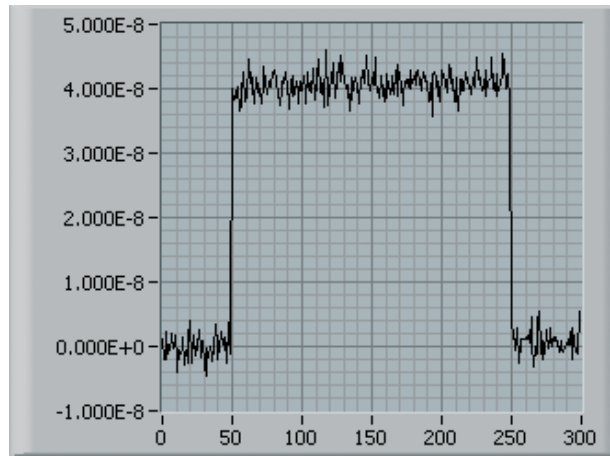
FIG 10: Power/time template of a nonrecurring RF burst for an application in medical electronics, measured with the R&S NRP-Z11 (LabView application without basic unit; readings in W and ms, no averaging).
