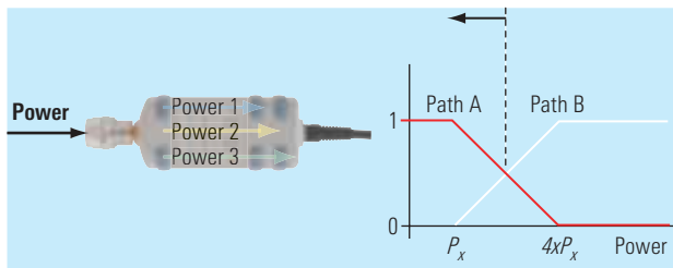
FIG 6: Parallel signal processing and soft transitions between measurement paths owing to R&S SMART SENSOR TECHNOLOGY .
