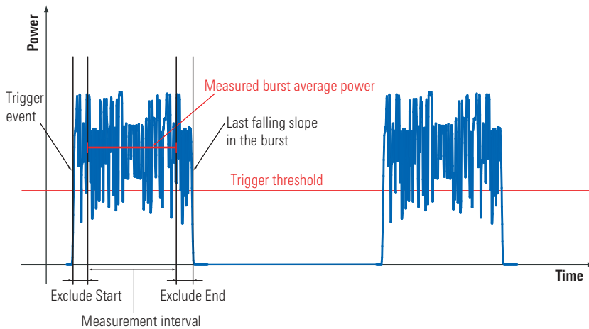
FIG 8: Modulated burst of an EDGE signal and relevant parameters for measurement of most average power.
