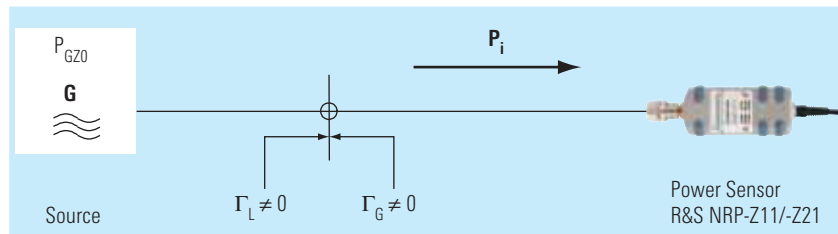
FIG 3: \Gamma correction function: By taking into account the complex reflection coefficient \Gamma_G of the source, the measurement result ( P_i ) is corrected in such a way that the nominal power P_{GZ0} of the source is displayed.
