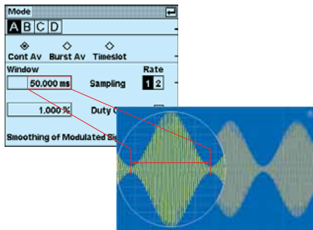
FIG 7: Windowing technique used on a low-frequency AM signal.
